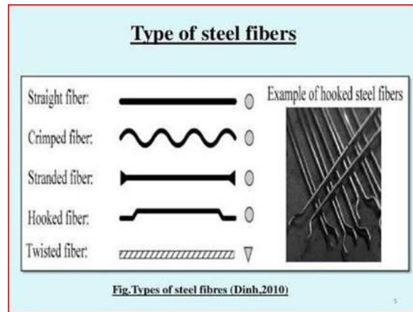
Figure 1. Types of steel fiber
